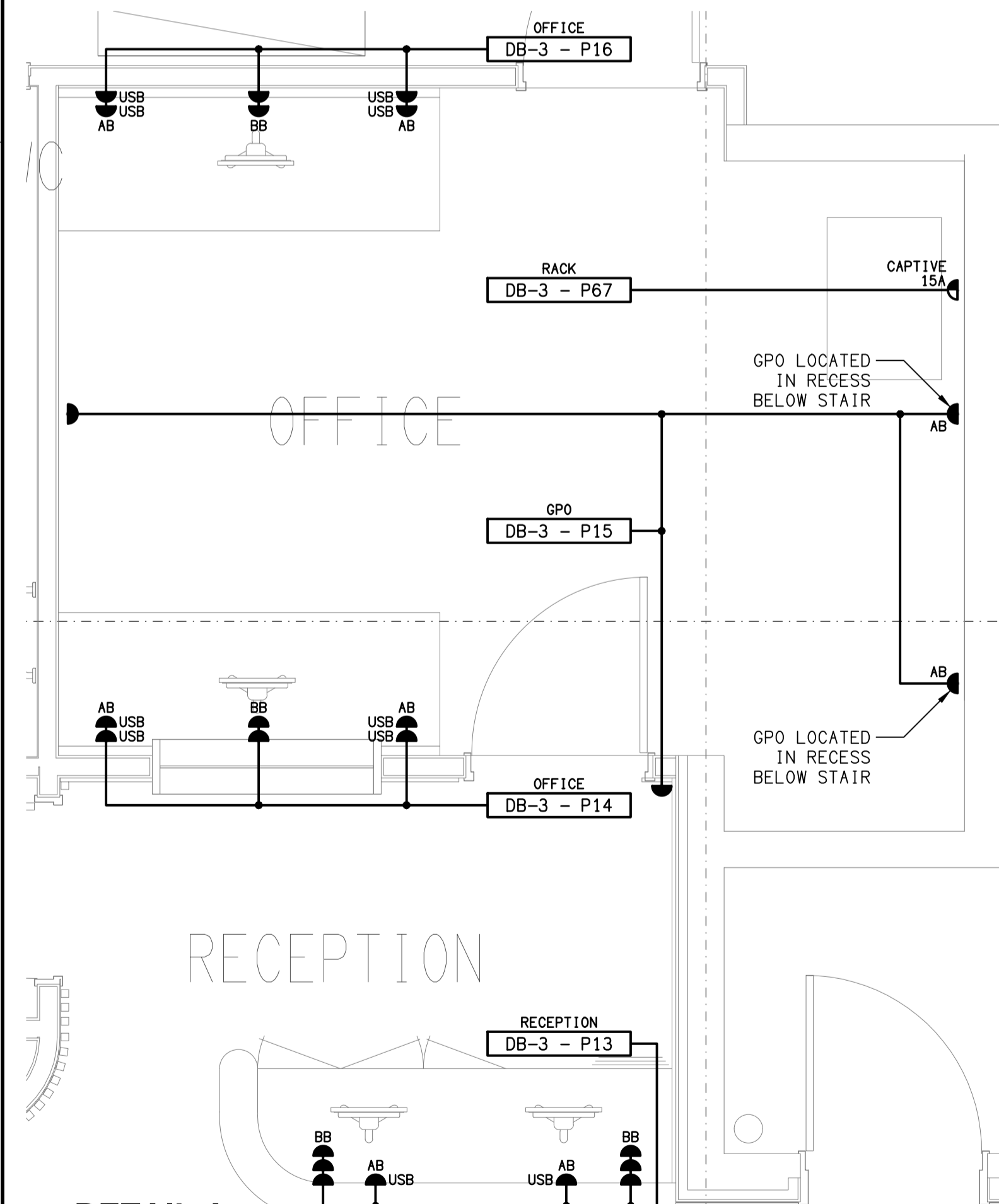
DETAIL A OFFICE / RECEPTION FLOOR PLAN SCALE 1:25
